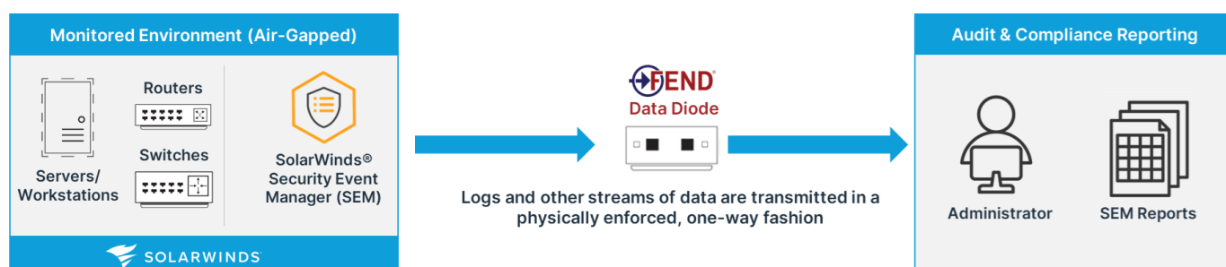
Figure 1: Fend – SolarWinds SEM Architecture Monitored Environment (Air-Gapped)
